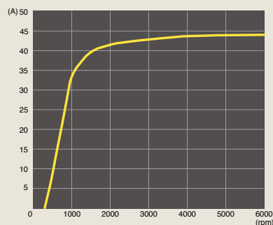
Alternator Output
